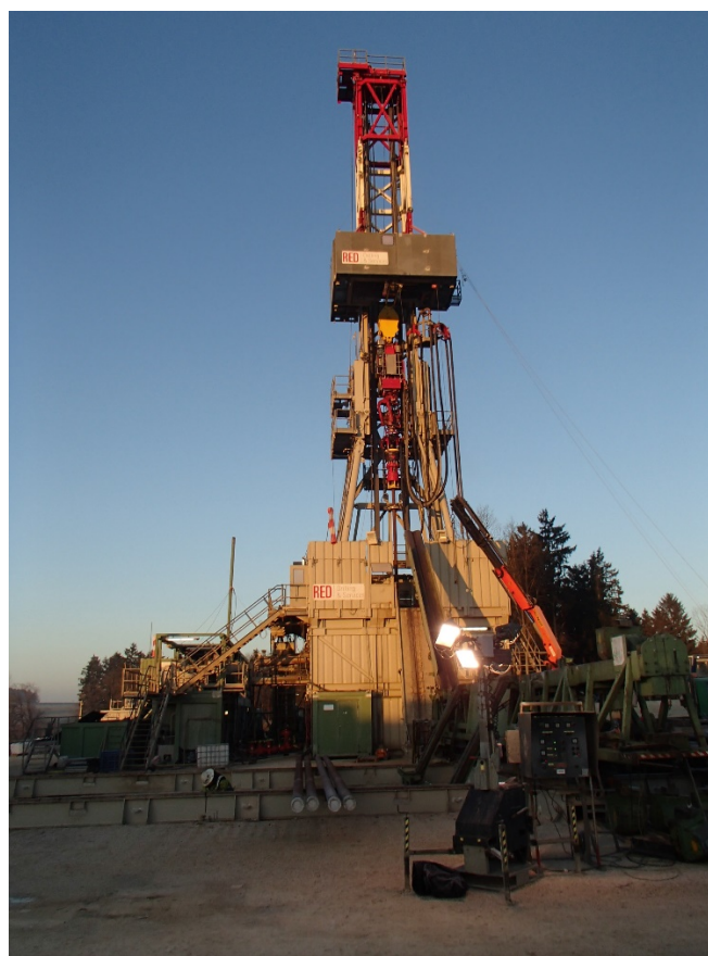
Figure 1: Running casing using the RED E-200 rig at the Anshof-3 drill site
